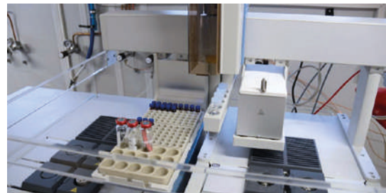
Non-targeted screening
