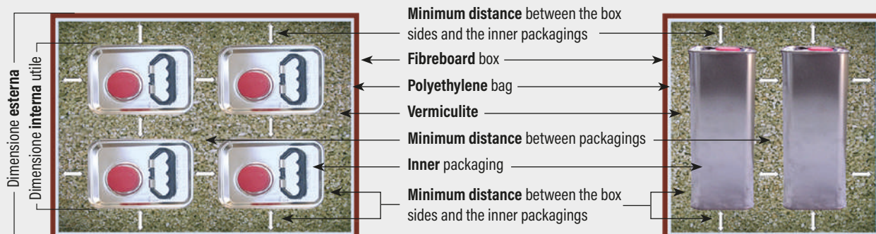
4 Insert the absorbent and cushioning material (Vermiculite) up to the top of the box, as to completely fill the polyethylene bag.
