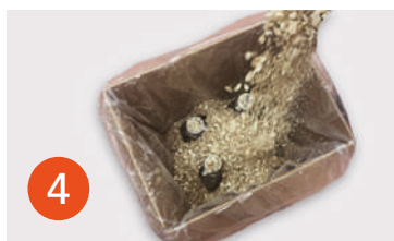
4 Insert the absorbent and cushioning material (Vermiculite) up to the top of the box, as to completely fill the polyethylene bag.
